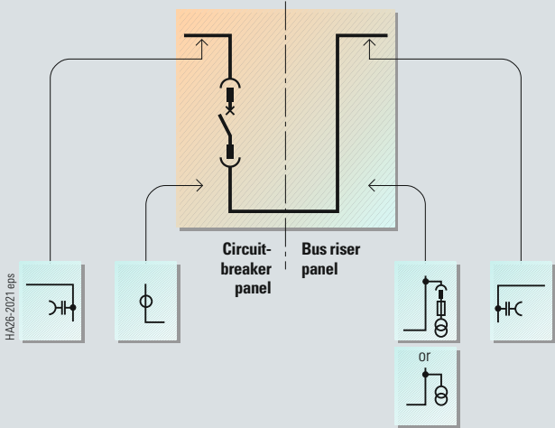
Bus sectionalizer (mirror-image installation also possible)
